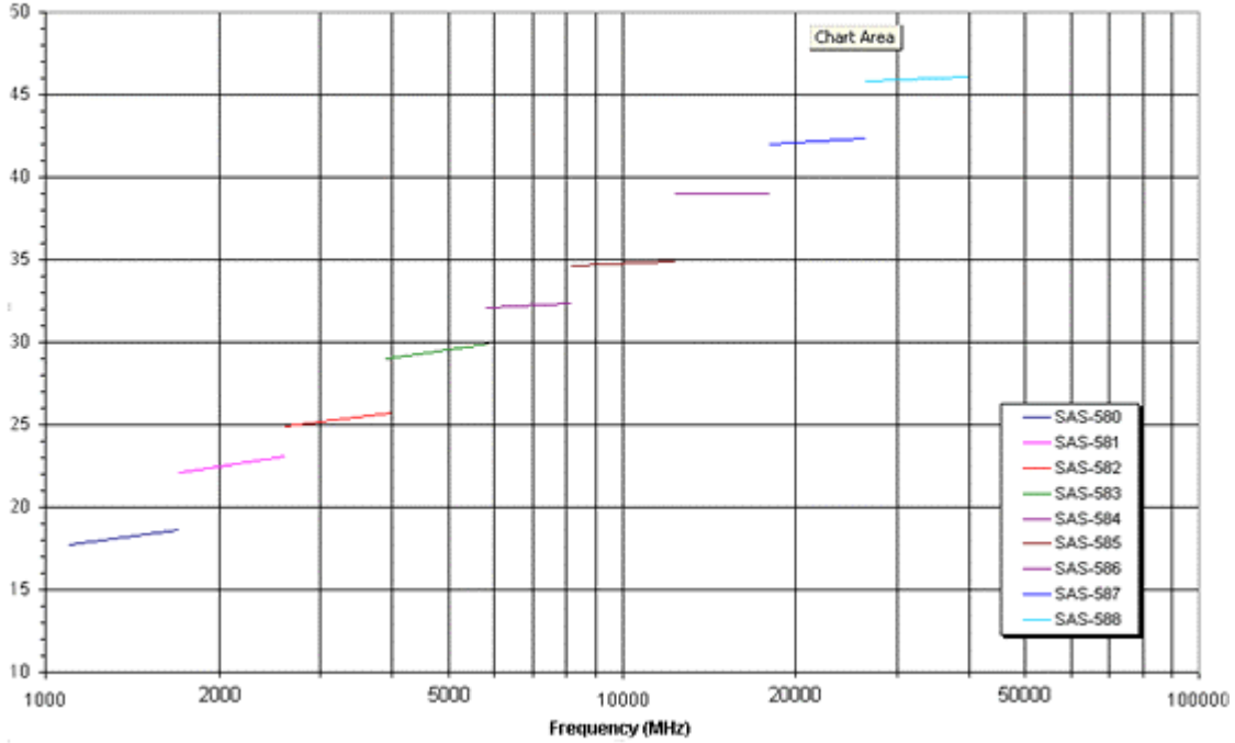
Standard Gain Horns Antenna Gain (dBi)
